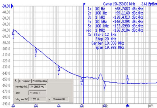
Frequency 156.250MHz
