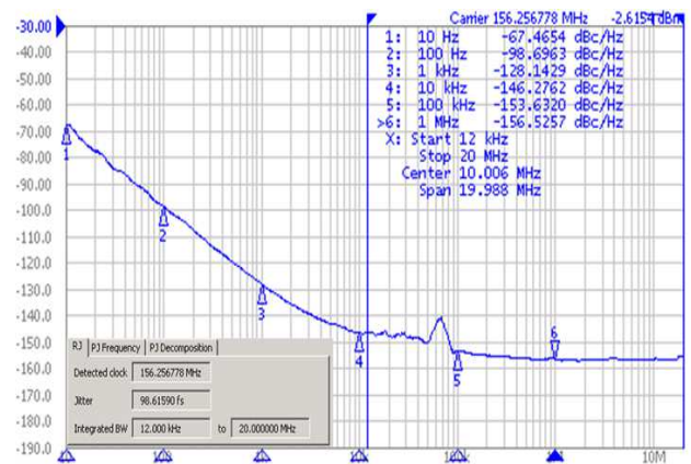
Frequency 156.250MHz
